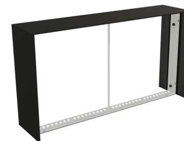
200x110cm - lada Modularico M100LED, wysoka dwustronna, czarna 200 × 50 × 110 cm · LAD-M100LED-200C-WD
